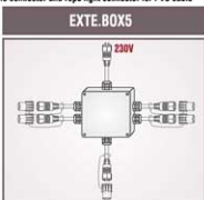
Easy Fix box with 5 outputs for rubber cable light string *For LED, use only with the reference CONVERTOR.LED.FL
