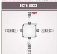
Easy Fix box with 3 outputs for rubber cable light string *For LED, use only with the reference CONVERTOR.LED.FL
